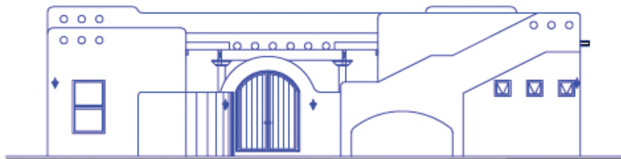
FRONT ELEVATION 3
